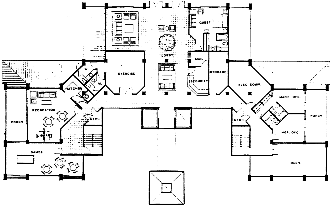
LOBBY FLOOR PLAN
